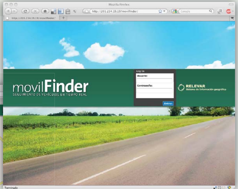
PANTALLA PRINCIPAL
